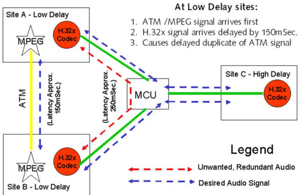
Transmission Echo Figure C - Echo caused by copies of the same signal
